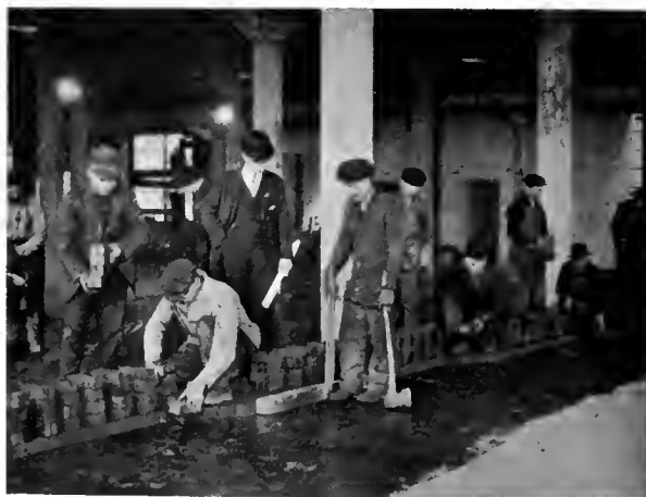
LAYING A WOOD BLOCK FLOOR
